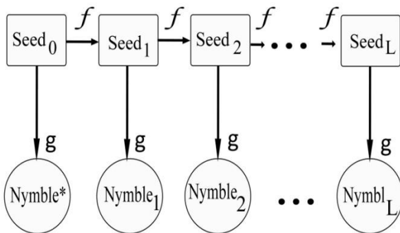
Fig. 2. Evolution of seeds and nymble
