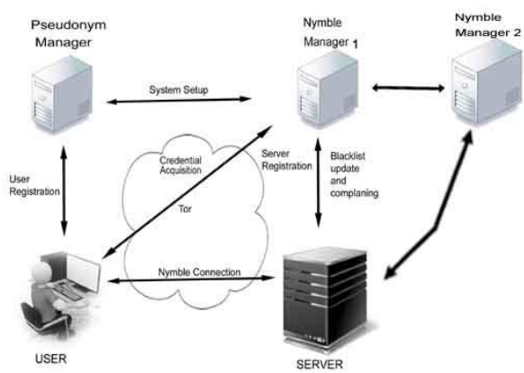
Fig @The Nymble system architecture
